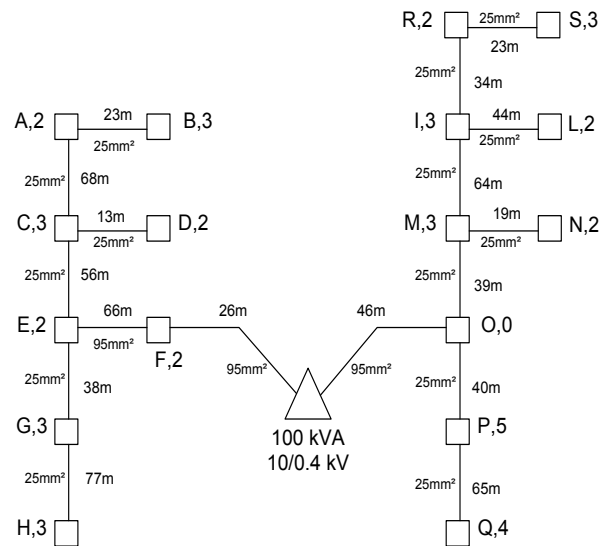
Fig. 2. Residential LV grid
