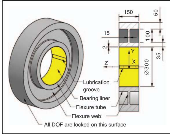
Figure 1. Flexure journal bearing geometry and system coordinates. DOFs: degrees of freedom.
