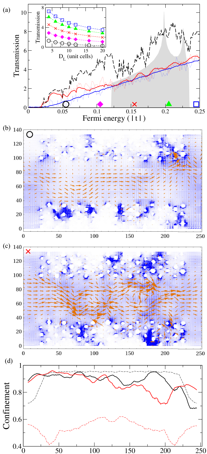
FIG. 12. (Color online) (a) Transmission through a D_L = 10 waveguide composed of pristine \{7,3,0\}_C antidots (black, dashed) or with S = |t| edge roughness (red) or \delta_{xy} = a , \delta_r = a geometric disorder (blue) applied. The dotted curves represent single configurations and the solid curves configurational averages. Grey shading shows the bulk GAL density of states. The inset shows the dependence on device length for different energies for the geometric disorder case. (b) and (c) show LDOS and current maps through a geometrically disordered sample at E_F = 0.05|t| and E_F = 0.15|t| , respectively. (d) Solid lines show the confinement along the length of the device for the energies in (b) (black) and (c) (red). The dashed lines show the confinement for the corresponding pristine systems.
