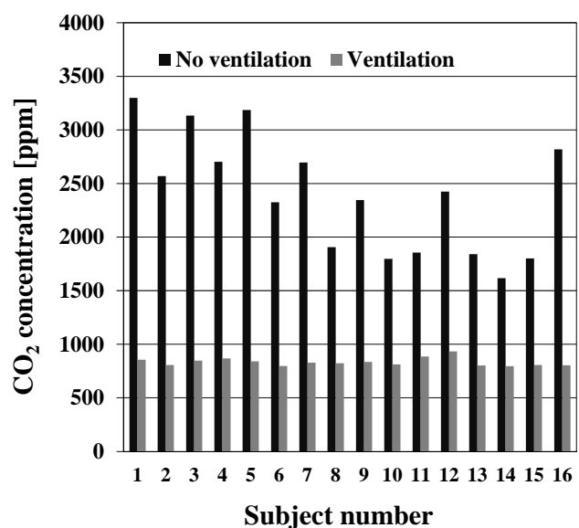
Figure 2: Comparison of the CO 2 concentration during night-time, each bar representing a 4-day average
