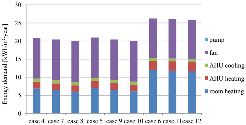
Fig. 6 Energy demand for different occupancy profiles and DPV fan power at indoor temperature of 29 °C
