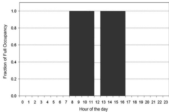
Fig. 2 Occupancy profile 1
