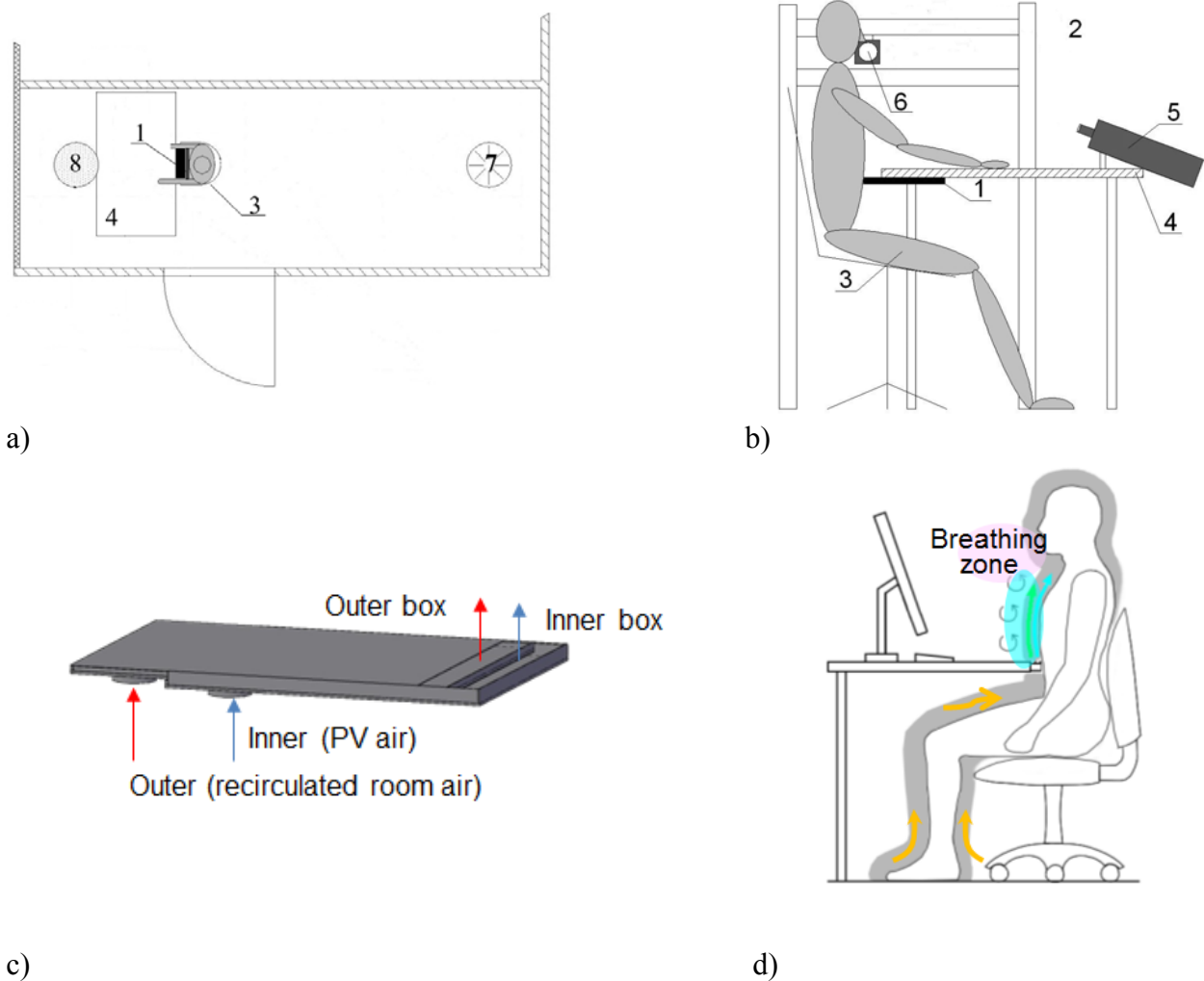
Figure 1. PIV set-up of the experiment with the confluent PV jet box a) chamber set-up and b) closer side view. 1) PV box with confluent jets, 2) stand, 3) thermal manikin, 4) table, 5) laser generator, 6) CCD cameras, 7) TV supply, 8) TV exhaust c) confluent PV jet design, d) application of confluent jets as a table incorporated PV unit.
