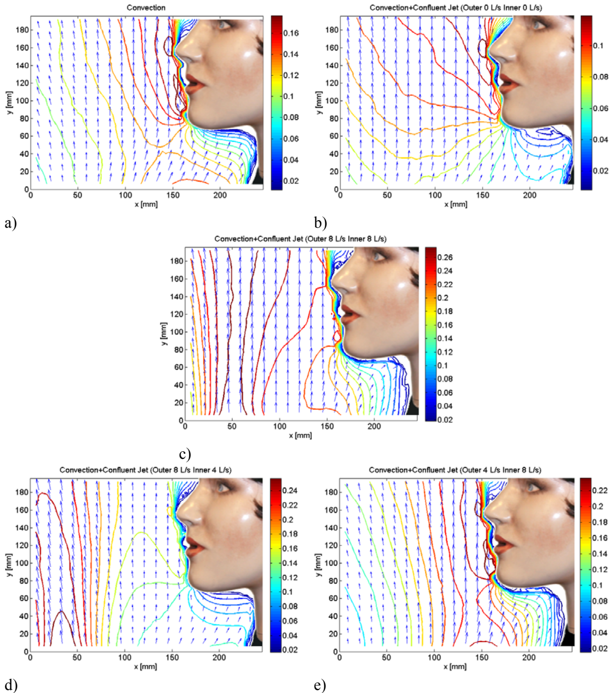
Figure 2 Vector and contour plots of velocity field in the x, y plane bisecting the manikin measured with the PIV when a) there was 0.12 m air gap between the manikin and the table, b) the confluent PV jet design was installed but not operational (used as an obstacle), c) both slots supplied 8 L/s upwards, d) the outer slot supplied 8 L/s and the inner slot (closer to body) supplied 4 L/s, e) the outer slot supplied 4 L/s and the inner slot (closer to body) supplied 8 L/s.
