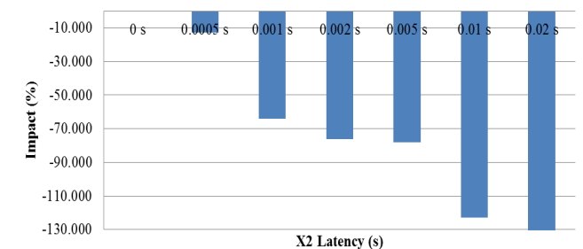
Fig. 8. Impact of X2 Latency on Ideal CoMP JT Gain
