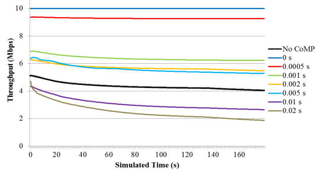
Fig. 5. Throughput of Pedestrian UE varying the X2 Latency
