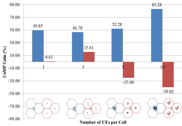
Fig. 3. System Throughput Gain vs System Load and UE Distribution
