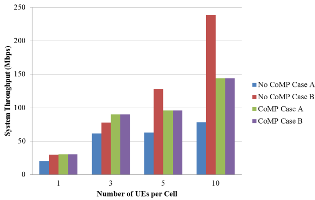
Fig. 4. System Throughput vs System Load and UE Location
