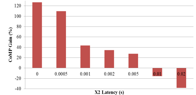
Fig. 7. System Throughput Gain vs X2 Latency
