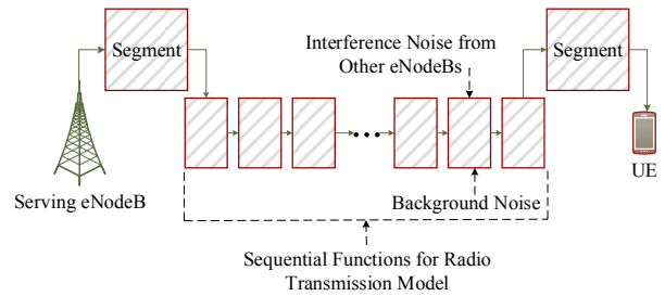
Fig. 2. Radio Transmission Model
