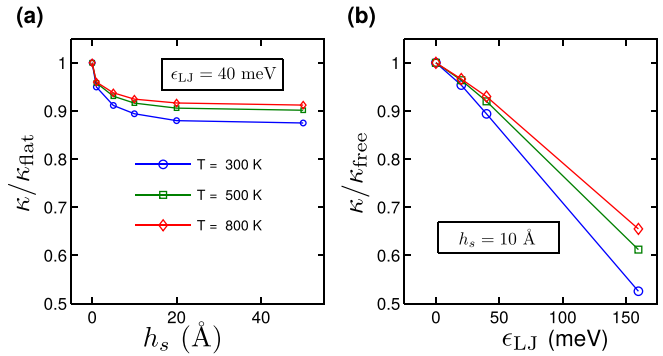
FIG. 4. The ratio of thermal conductance of graphene over a step for a fixed interaction strength ( \epsilon_{LJ} = 40 meV) as a function of the step height (a), and for a fixed step height ( h_s = 10 Å) as a function of the interaction strength (b).
