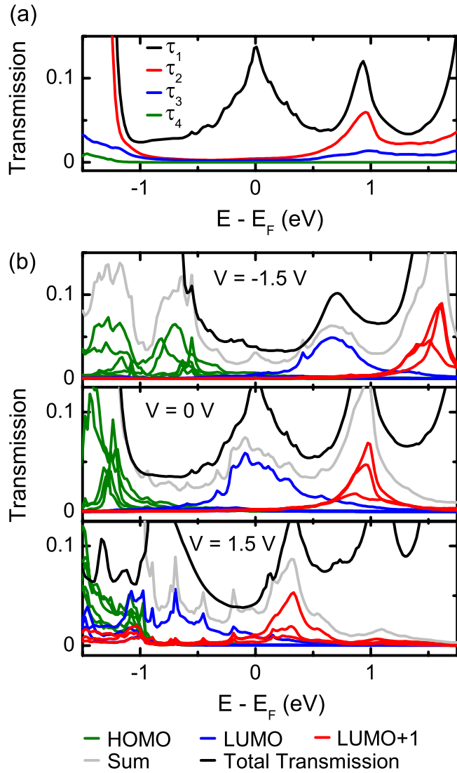
Figure 6. (a) Eigenchannel transmissions, \tau_n(E) ( n = 1, \dots, 4 ), at zero bias for the contact range (tip-C 60 distance: 1.9 Å) averaged over all k points. The dominant transmission channel (black, transmission probability \tau_1(E) ) closely follows the C 60 HOMO, LUMO, and LUMO+1. Around the energy of the LUMO+1 ( \approx 0.9 eV) three channels contribute to the conductance. (b) Orbital-projected transmission functions T_\alpha(E) for the C 60 HOMO (green), LUMO (blue) and LUMO+1 (red) resonances evaluated at the indicated voltages (tip-C 60 distance: 1.9 Å, i.e. in the contact range). Several contributions are observed from each orbital due to their partial degeneracy. The grey line depicts the sum of all transmissions, \sum_\alpha T_\alpha(E) , while the solid black line is the total transmission calculated according to equation (1).
