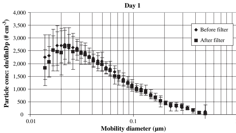
Fig. 2. Performance of the prefilter on Day 1, determined by the SMPS. Error bars represent standard deviations.
