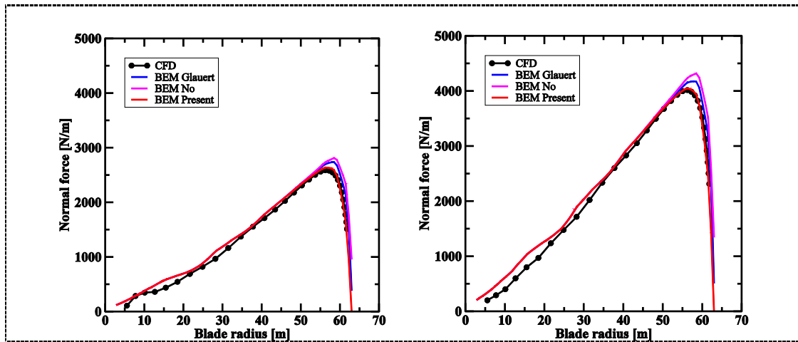
Figure 8. Normal force on the NREL 5MW turbine at a wind speed of 6 m/s (left) and 8 m/s (right)
