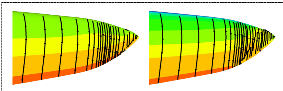
Figure 2. Limiting streamlines in the tip region of a LM19.1 blade at wind speeds of 7 (left) and 12 (right) m/s.
