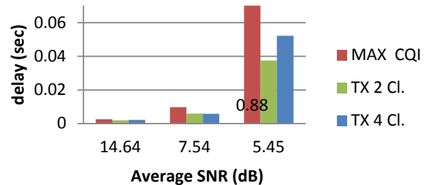
Figure 10: Video average delay
