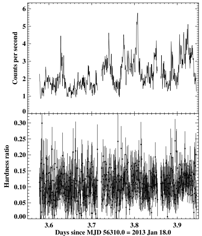
Figure 2. Top panel: background-subtracted 0.3–10 keV light curve of Cen X-4 measured with XMM-Newton /EPIC-pn, binned at 50 s resolution. The typical error bar is \pm 0.16 \text{ counts s}^{-1} . The short data gaps are intervals that were excluded owing to strong background flares. The source intensity shows strong flaring behavior, varying by more than a factor of two on timescales as short as a few minutes. The brightest flare, around MJD 56313.8, is also visible in the NuSTAR light curve (see Figure 1). Bottom panel: spectral hardness of the count rate shown in the top panel, constructed by taking the ratio of the 2–10 keV and 0.3–1.0 keV count rates. There is no evidence for significant spectral changes during the flaring intervals, although there is weak evidence for a small change during the flare at MJD 56313.63.
