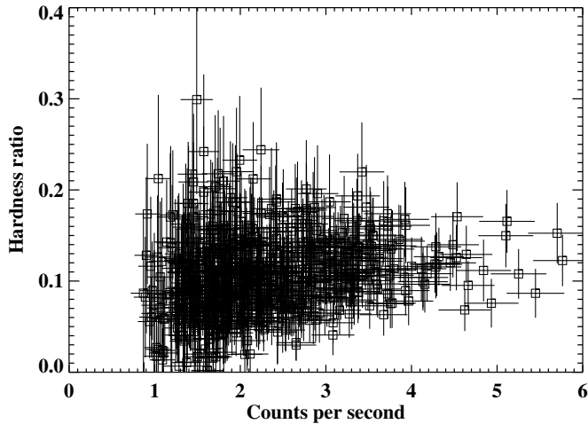
Figure 3. Hardness–intensity diagram for XMM-Newton /EPIC-pn observation of Cen X-4. The x axis shows the 0.3–10 keV count rate, and the y axis shows the spectral hardness (defined as the ratio of the 2–10 keV and 0.3–1.0 keV count rates). There is no evidence for significant spectral changes as a function of source intensity.
