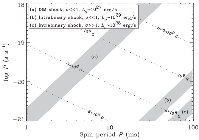
Figure 7. Regions with low predicted cutoff energy E_c for a synchrotron shock spectrum, displayed as a function of the radio pulsar spin period P and period derivative \dot{P} ; P and \dot{P} are not known for Cen X-4. The dotted lines show contours of constant pulsar magnetic field strength B (see Equation (12)). The shaded regions have E_c in the 5–20 keV range, consistent with the observed power-law cutoff energy in Cen X-4, and correspond to the three cases listed in the box on the upper left. Radiative losses are negligible in all of these regions ( \gamma_s > \gamma_m ). Contours of constant E_c and constant synchrotron luminosity L_s have the same slope on the P – \dot{P} plane. In all three regions, the predicted L_s is orders of magnitude too small to explain the observed power-law luminosity ( \sim 10^{32} erg s^{-1} ) in Cen X-4. Additional regions, corresponding to the intrabinary shock cases where radiative losses dominate ( \gamma_s < \gamma_m ), are not shown; they lie in an unphysical part of the phase space ( P \lesssim 1 ms and B \gtrsim 10^9 G) for E_c < 20 keV. All calculations were done with \eta_V = 0.3 , \epsilon_a = 0.2 , and f_{\text{geom}} = 0.05 .
