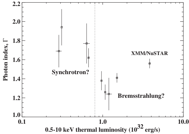
Figure 8. Hard X-ray power-law photon index (2–10 keV) vs. unabsorbed 0.5–10 keV thermal luminosity for deep observations of Cen X-4 (see Table 3). The XMM/NuSTAR point is from a tbabs*(nsatmos+powerlaw) fit to the 0.3–10 keV data only. The thermal luminosity L_{\text{th}} is computed for a distance of 1 kpc. For L_{\text{th}} \gtrsim 10^{32} D_{\text{kpc}}^2 \text{ erg s}^{-1} , the data are roughly consistent with a trend of steeper power-law slope for higher L_{\text{th}} , as expected for bremsstrahlung emission, if we assume that kT_e is reduced from 50–100 keV via Compton cooling by thermal photons. In energy bandpasses well below kT_e , a bremsstrahlung spectrum is a \Gamma = 1 power law. The large \Gamma measured at the lowest thermal luminosities may indicate a transition to synchrotron shock emission at extremely low \dot{M} .
