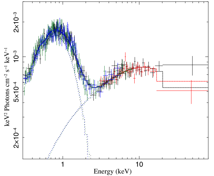
Figure 6. Unfolded \nu F_{\nu} spectrum of Cen X-4 corresponding to the \text{tbabs}*(\text{nsatmos}+\text{bremss}) fit shown in Figure 5. The individual model components are denoted by the dotted lines. The cutoff of the hard spectral component above 10 keV is clearly visible.
