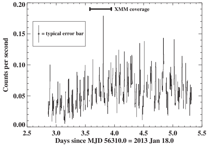
Figure 1. Background-subtracted 3–20 keV light curve of Cen X-4 measured with NuSTAR , binned at 300 s resolution. The average of the FPMA and FPMB count rates is plotted, and the size of a typical error bar is shown. The data gaps are due to Earth occultations. The source intensity varies significantly on timescales of minutes to hours. The interval with simultaneous coverage with XMM-Newton is indicated and includes a bright flare around MJD 56313.8 (see Figure 2).
