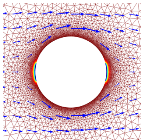
Figure 1: (Left) NAPL-FLUTE liner (a color striped membrane) in combination with the activated carbon strip (FACT). (Right) Simulation results showing two FACTs in a borehole after an exposure time of 42 h in an aquifer with an initially uniform dissolved PCE concentration. The blue arrows mark the groundwater flow velocity.
