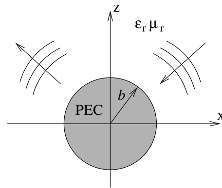
Fig. 6. Scattering of a spherical wave by a PEC sphere immersed in a medium with parameters \varepsilon_r , \mu_r , k_s = \sqrt{\varepsilon_r \mu_r} k , \lambda_s = 2\pi/k_s .
