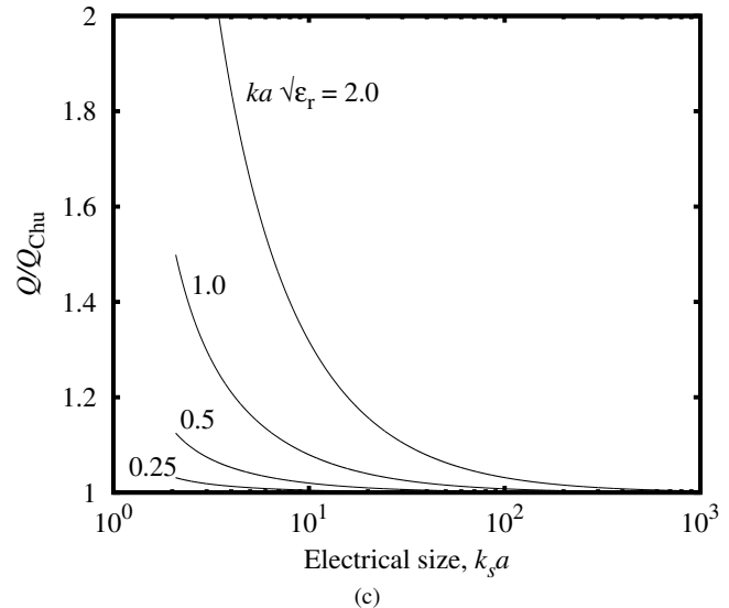
Fig. 4. Optimal relative radius of the PEC core b/a (a) and the corresponding lowest achievable ratio Q/Q_{\text{Chu}} : (b) for n = 1, 2, 3 , and ka\sqrt{\epsilon_r} = 1.0 ; (c) for various ka\sqrt{\epsilon_r} and n = 1 .
