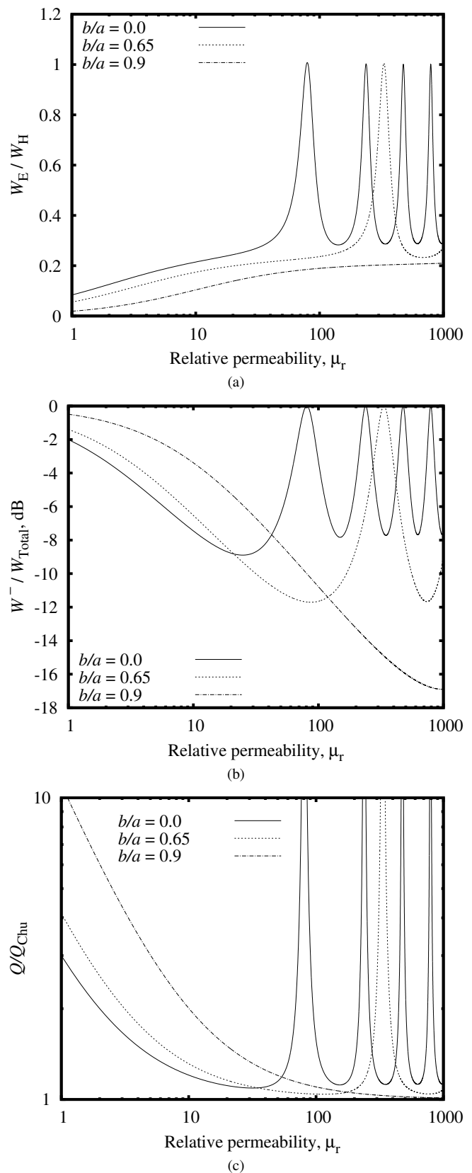
Fig. 2. Energy and quality factor as functions of \mu_r ( \epsilon_r = 1 ) for fixed ka = 0.5 : (a) Ratio of electric and magnetic stored energies; (b) Ratio of internal and total stored energy; (c) Quality factor (normalized by Chu lower bound).
