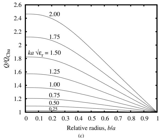
Fig. 3. Optimal electrical size k_s a (a) and the corresponding lowest achievable ratio Q/Q_{\text{Chu}} : (b) for n=1, 2, 3 , and ka\sqrt{\varepsilon_r} = 1.0 ; (c) for various ka\sqrt{\varepsilon_r} and n=1 .
