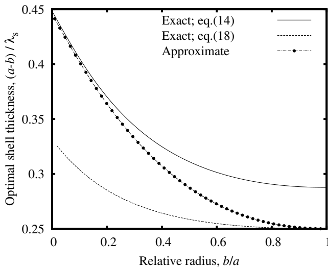
Fig. 7. Exact and approximate optimal thickness of the shell.
