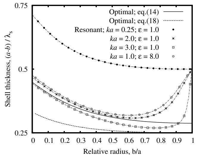
Fig. 5. Optimal shell thickness and shell thickness for the first resonance.
