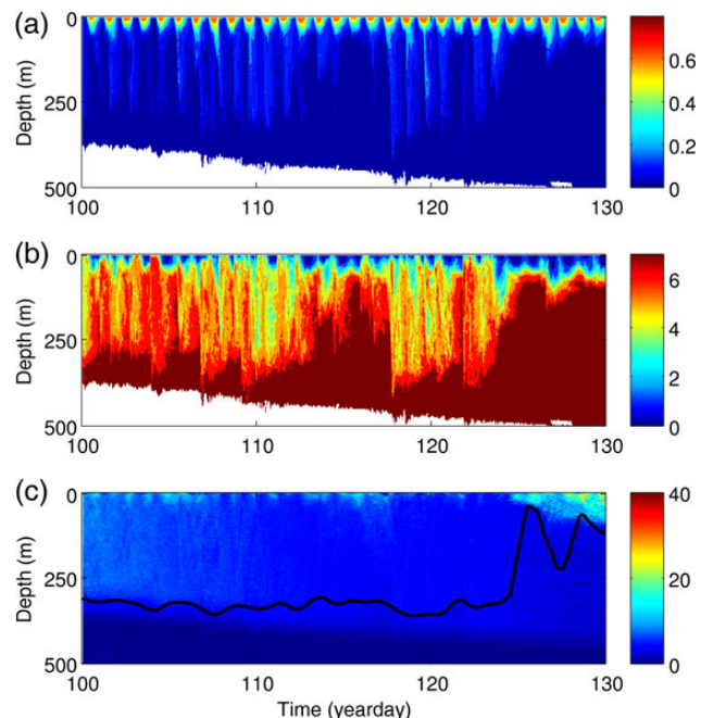
Figure 3. Phytoplankton properties simulated by the non-hydrostatic CM over the course of the simulation at Ocean Weathership Mike. Hovmöller diagrams show the (a) carbon-specific respiration rate ( \text{d}^{-1} ), (b) sinking rate ( \text{m d}^{-1} ), and (c) phytoplankton concentration ( \text{mg C m}^{-3} ).
