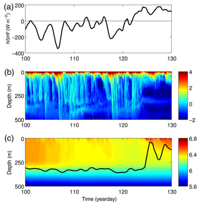
Figure 1. Physical water properties as predicted by the non-hydrostatic CM over the course of the simulation at Ocean Weathership Mike. (a) Simulated net surface heat flux ( W m^{-2} ). (b) Hovmöller diagram showing simulated water column TKE ( cm^2 s^{-1} ) on a log scale. (c) Simulated temperature within the water column ( ^{\circ}C ). The black line indicates the estimated mixed-layer depth.
