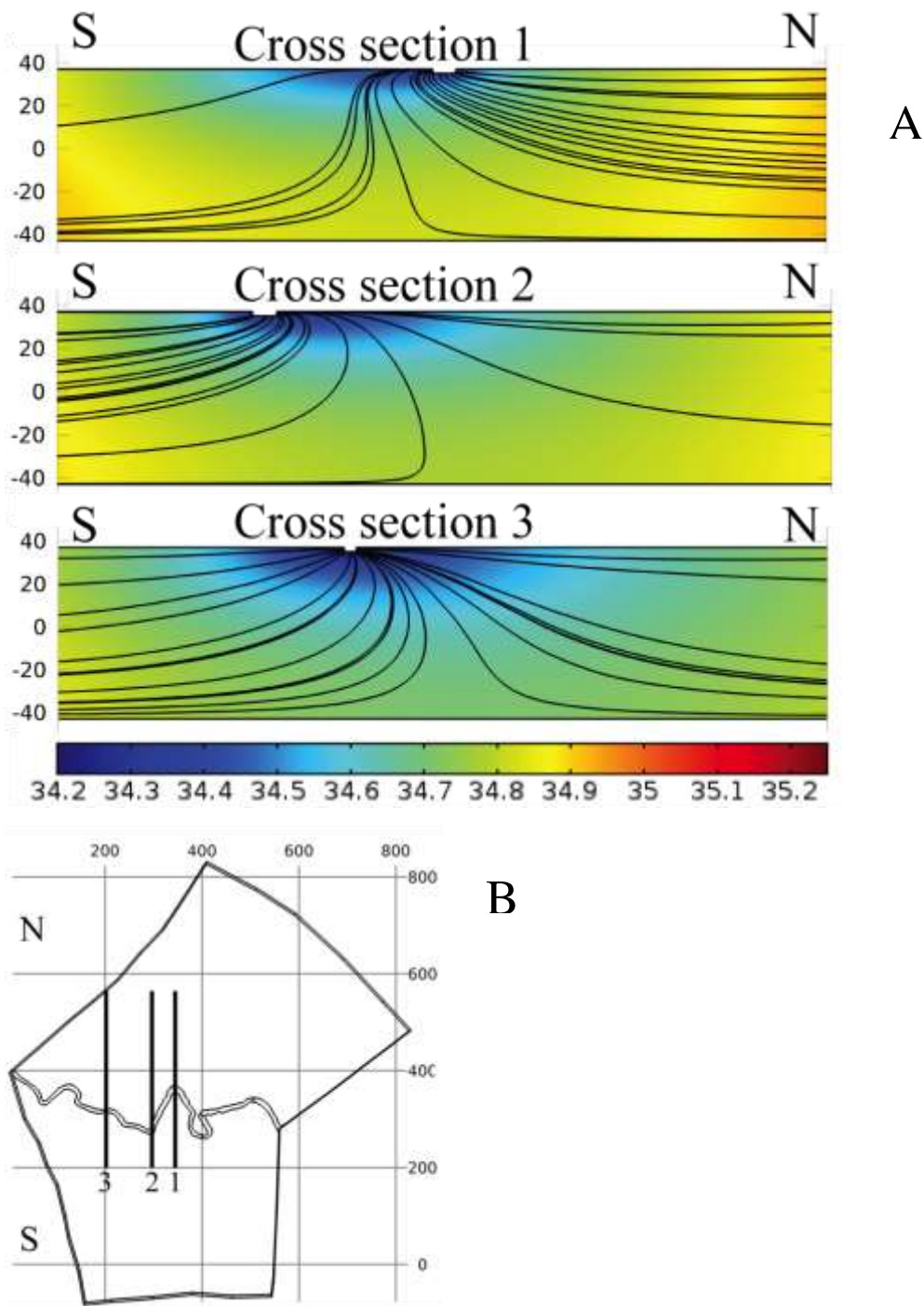
Figure 1: Cross sections of Grindstedt Å (Panel A), showing modelled head (m) and groundwater streamlines toward the stream. Panel B shows the location of the cross sections. As can be seen in cross section 1, most of the water discharging to the stream comes from the area north of the stream. In contrast, groundwater water flowing to the stream at cross section 2 comes from the south.
