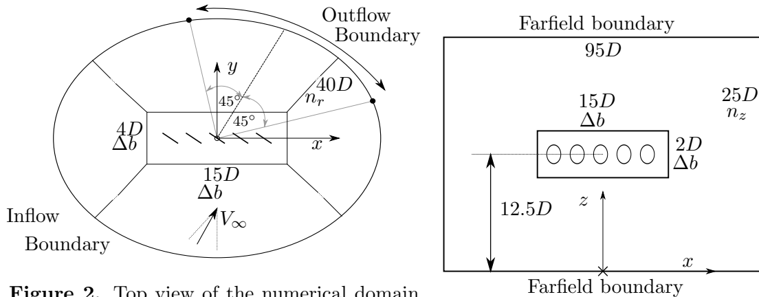
Figure 2. Top view of the numerical domain. All dimensions are scaled by the turbine diameter D . Note that the boundaries are a function of the inflow angle.
