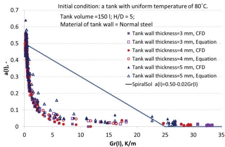
Fig. 6 the heat removal factors for a 150 l normal steel tank with different tank wall thicknesses.
