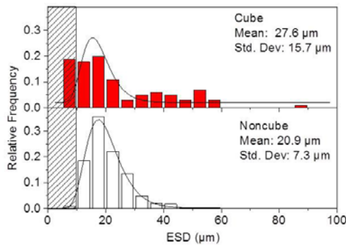
Fig. 2 Size distributions of cube and noncube grains at the end of the measurement ( \sim 25\% recrystallized). There are more cube grains smaller than 10 \mu\text{m} , because of the different detection limits for cube and noncube grains (see text in Section 3 for details). To avoid this bias, a cut-off size of 10 \mu\text{m} was used, i.e. grains in the shaded part are not included in the following analysis. The size distributions of grains larger than 10 \mu\text{m} were fitted to lognormal functions.
