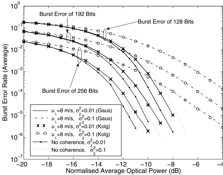
Fig. 6. Burst error rate against normalized average optical power for OOK format with a 25 % duty cycle for \sigma_{\chi^2} = 0.1 and 0.01 and for u_{\perp} = 8 m/s and no coherence ( u_{\perp} \rightarrow \infty ). The burst error length is established to 256, 192 and 128 bits (Jurado-Navas et al., 2007).
