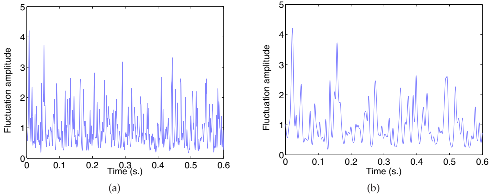
Fig. 7. Time-varying atmospheric scintillation sequence, \alpha_{sc}(t) generated for an average wind speed transverse to the direction of propagation of a) u_{\perp} = 8 m/s. b) u_{\perp} = 2.5 m/s.
