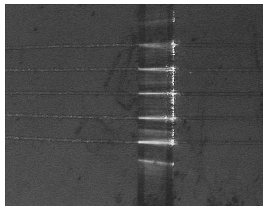
Fig. 2: Five waveguides spanning a 500 μm wide flow channel. Light from an argon-ion laser is coupled into the channel and excites the fluorescein solution in the channel.
