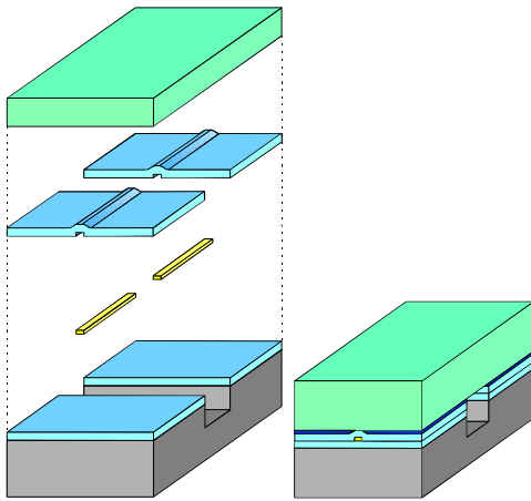
Fig. 1: This figure shows the microsystem with the silicon part, the three layers of glass and the Pyrex part in exploded and normal view.
