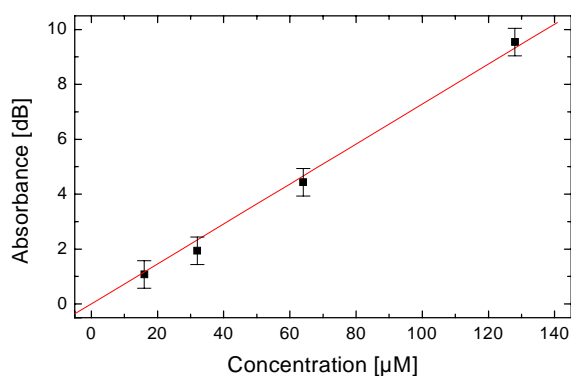
Fig. 3: Absorbance versus different concentrations of Fluorescein. Measuring wavelength is 488 nm
