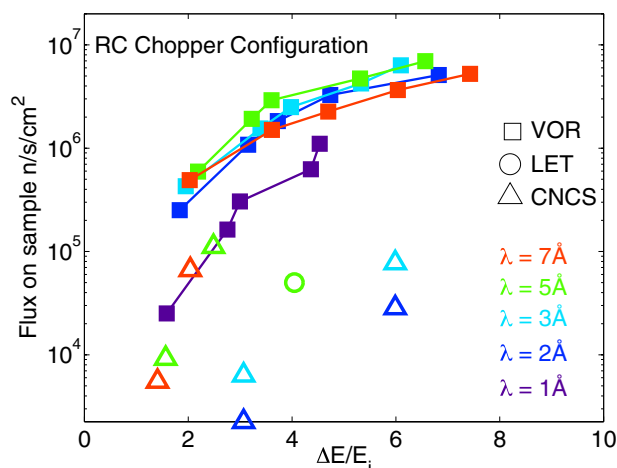
Figure 7. Neutron flux on sample as a function of energy resolution for a range of incident wavelengths for the relative constant energy resolution chopper configuration.
