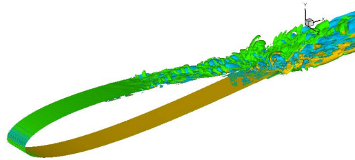
Figure 3. Iso-vorticity plot.
