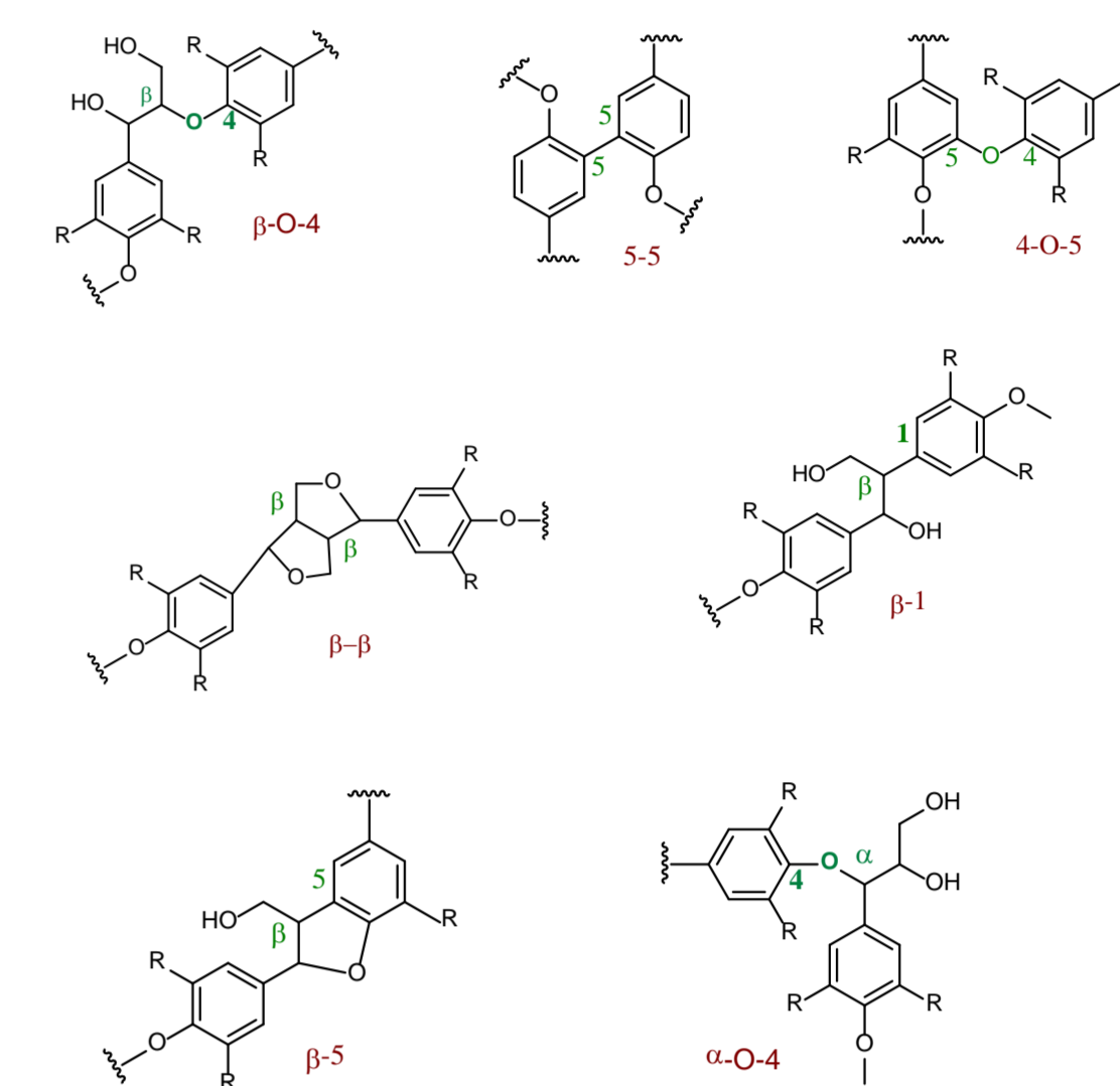
Figure 2. Type of bonds in lignin.
