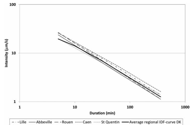
Figure 4 | IDF curves for the best five French stations compared to the current regional average IDF curve in Denmark for a return period of 2 years.
