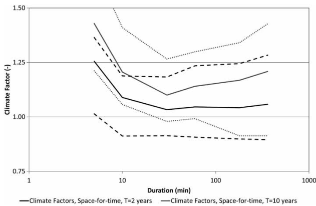
Figure 5 | Calculated mean climate factors for each duration for return periods 2 and 10 years based on the five French stations. Solid lines indicate mean values, and dashed and dotted lines indicate the maximum and minimum climate factor for 2 and 10 year return periods, respectively.
