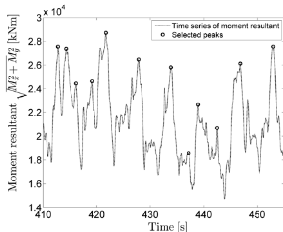
Figure 1: Example of load peaks extracted from simulated time history for blade bending moments M_x and M_y .
