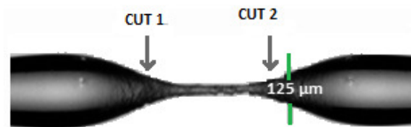
Figure 3: Tapered fibers cut at indicated position and polished to get CPC tips.
