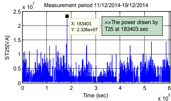
Figure 5-2: Load consumption at KAM T25 (at PCC) during one week period.
