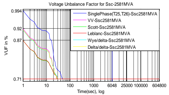
Figure 6-2: VUF (%) for different transformer connections introduced by load at SSP=2581MVA
