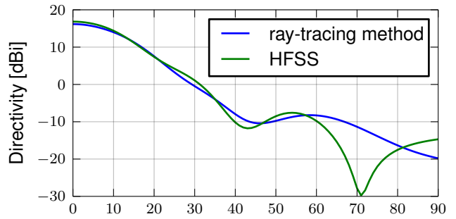
(a) \phi = 0^\circ (H-plane) \theta [deg]
