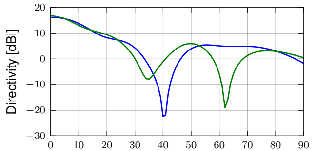
(c) \phi = 90^\circ (E-plane) \theta [deg]
