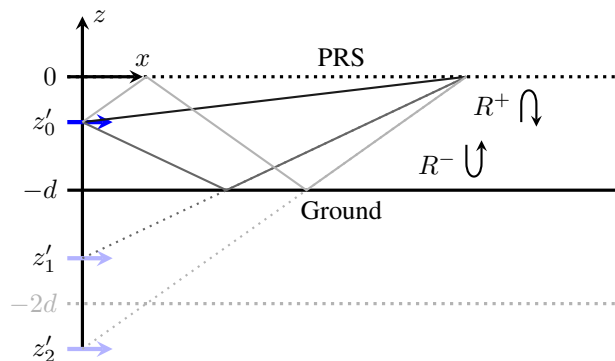
Fig. 1: An x -directed magnetic dipole located in a slab defined by complex plane wave reflection coefficients, R^+ , R^- , and the transmission coefficient T^+ .
