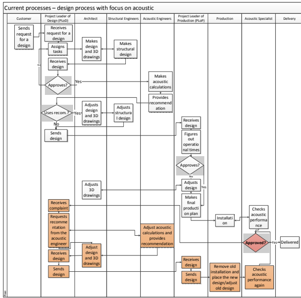
Fig. 1. Analysis of the current process: acoustic design processes in construction.
