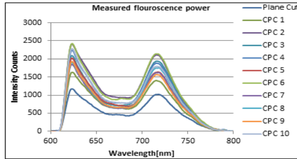
Fig. 12. Fluorescent spectrum for assay and reference fluorescence of batch 1 and plane cut fiber tip.
