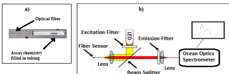
Fig. 11. (a) Dummy sensor (b) Setup for optical characterization of the CPC based sensor.
