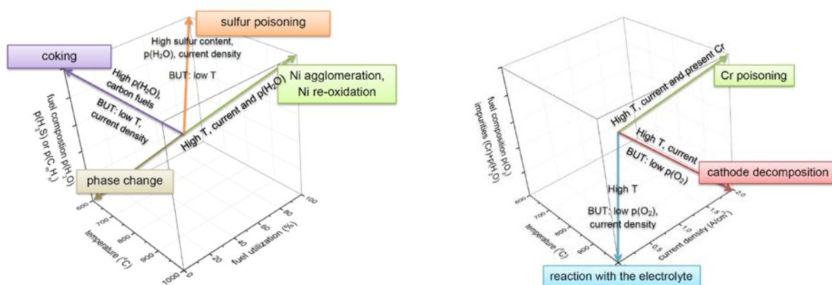
Fig. 1 Dependency of anode and cathode degradation mechanisms (examples) on operating parameters.
