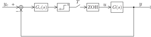
Figure 1. A linear system control by a relay.
