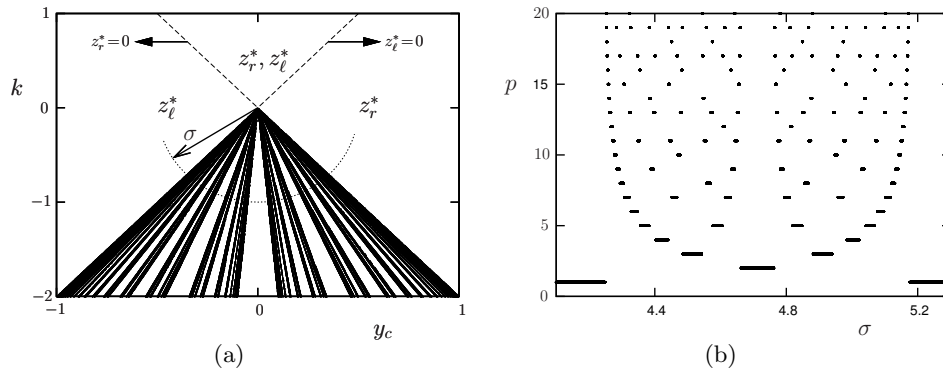
Figure 2. (a) Big bang bifurcation in the (y_c, k) parameter space for a = -2 , b = 1 and T = 0.1 . The fixed points z_i^* are labeled in the regions where they are feasible, and, as dashed lines, the border collision bifurcation curves where they become virtual are shown. The periods of the periodic orbits found along the pointed curve parametrized by \sigma are shown in (b).
