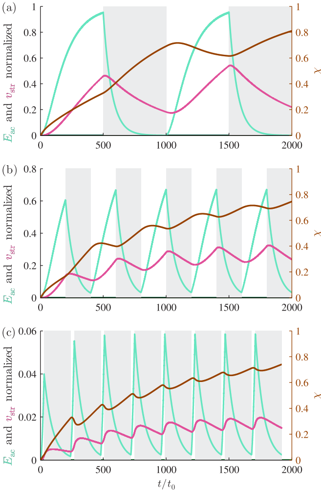
FIG. 8. (Color online) The same probes as in Fig. 7 but for the following pulsed actuation schemes: (a) actuation is on for 500 t_0 followed by no actuation for 500 t_0 repeatedly, (b) actuation is on for 200 t_0 followed by no actuation for 200 t_0 repeatedly, and (c) actuation is on for 30 t_0 followed by no actuation for 210 t_0 repeatedly.
