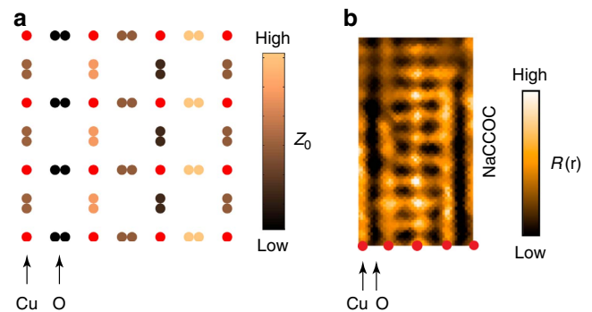
Figure 5 | Comparison of the bilayer oxygen height with an STM R(\mathbf{r}) image. (a) A representation of the spatial variation of the z c -ordinate of the bilayer oxygen atoms from our X-ray results is shown for one ( q_b ) of two modulation directions present in the crystal. In (b) is an STM R(\mathbf{r}) image, (where R(\mathbf{r}) = I(\mathbf{r}, E) / I(\mathbf{r}, -E) is a measure of the asymmetry of the current for positive and negative bias) acquired from the lightly doped cuprate \text{Ca}_{2-x}\text{Na}_x\text{CuO}_2\text{Cl}_2 (NaCCOC). (Reproduced with permission from ref. 22.) The R(\mathbf{r}) -image is used to highlight spatial variation of doping or electronic structure. Both (a) and (b) have the same symmetry as a bond d -density wave along the \delta_a direction. Note that NaCCOC has a repeat period of approximately four unit cells, which is longer than that in YBCO.
