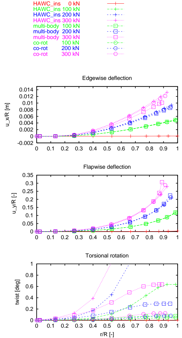
Figure 3: Calculated blade deflection shapes.
