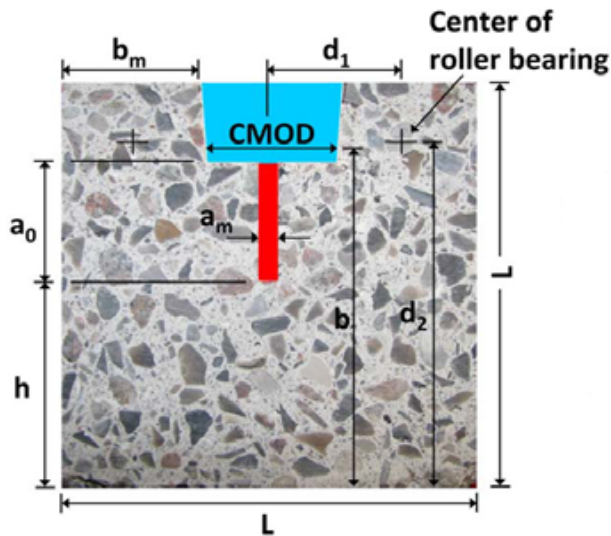
Fig. 3 WST specimen geometry with the blue area indicating the groove and the red area indicating 4.5 mm notch.
