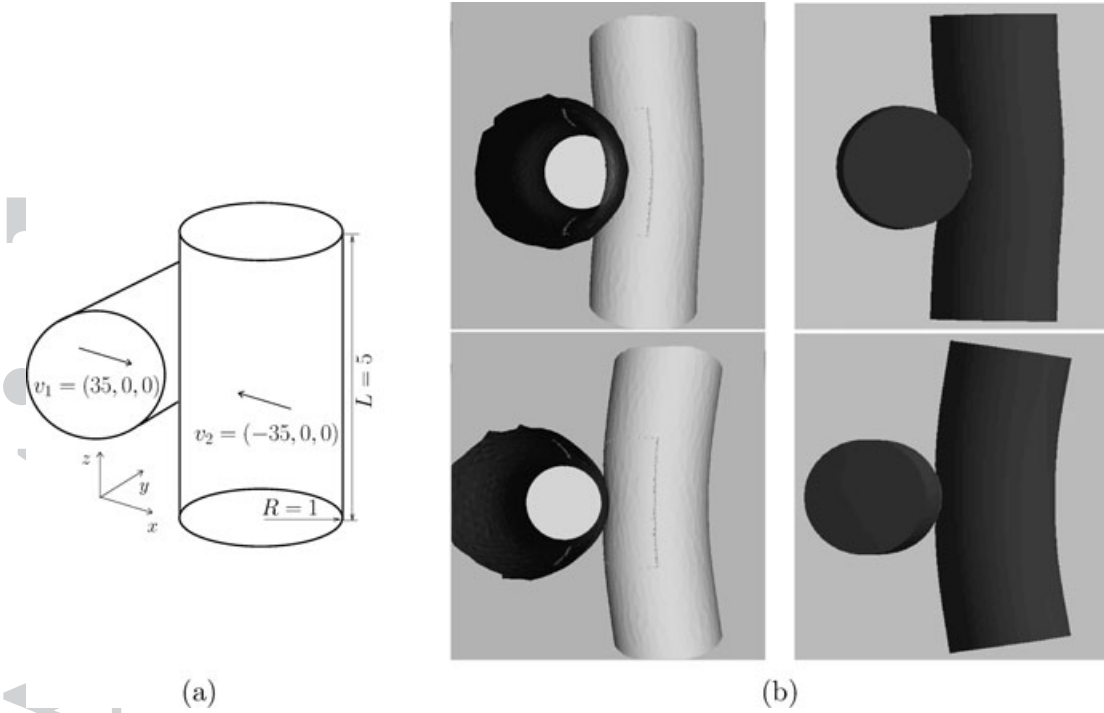
Figure 6. (a) Geometry of the impact problem. The origin is located at the center of the cylinder at the left of the illustration. All values in the SI of units. (b) Simulation of two colliding cylinders using the custom collision mechanism (left) and the commercial software ANSYS (right) at times t = 0.0011 s (top) and t = 0.003 s (bottom).
