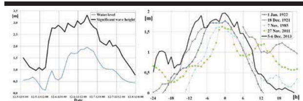
Figure 8. Measured significant wave heights and water levels at 7 m water depth during Xaver (A) and water levels (peak at 0 hrs.) at Hornbaek (solid black) (B) together with 'top-4' extreme water levels previous to this event.
