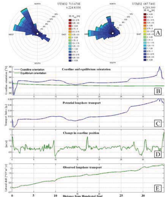
Figure 4. Modeled wave conditions off the coast (refer Figure 1 for positions) (A), coastline orientation and equilibrium orientation (B), calculated potential longshore transport (C), rate of change in coastline position (c. 1890-2005) (D), and observed longshore transport (E) for the Hundested to Gilleleje coastline.
