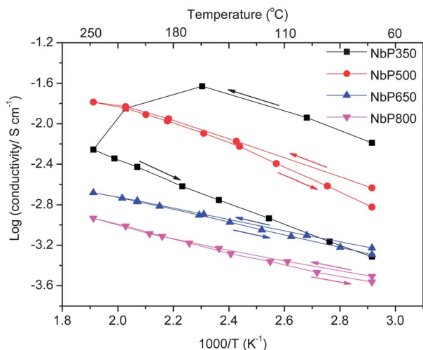
Fig. 5 Temperature dependence of conductivity for niobium phosphates under dry air. The arrows show the heating up and cooling down cycles of the measurements.
