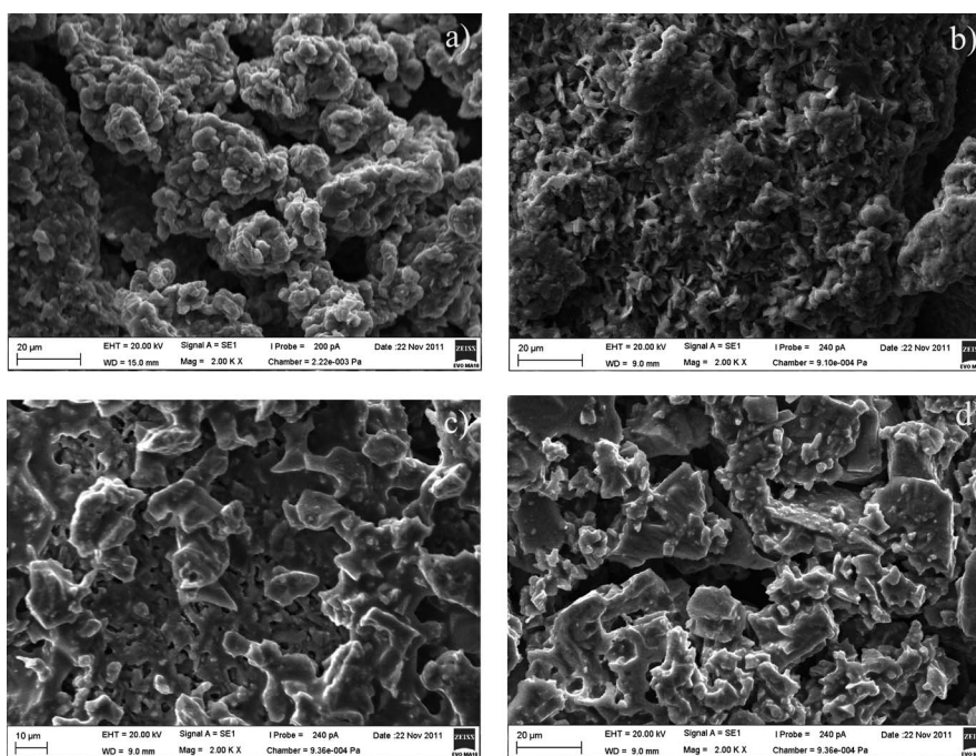
Fig. 4 SEM images of prepared niobium phosphate with different heat treatment temperatures: (a) 350 °C, (b) 500 °C, (c) 650 °C and (d) 800 °C.
