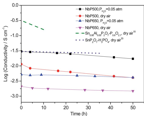
Fig. 7 Conductivity stability of NbP500 and NbP650 under dry air and humidified air with the water partial pressure of 0.05 atm at 250 °C. Dashed lines were taken from references as indicated in the figure.
