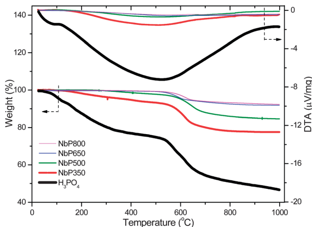
Fig. 3 TGA and DTA of the prepared niobium phosphates sintered at different temperatures and phosphoric acid.
