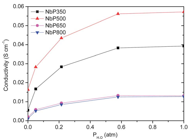
Fig. 6 Proton conductivity of niobium phosphates at 250 °C as a function of water partial pressure in the ambient pressure air.
