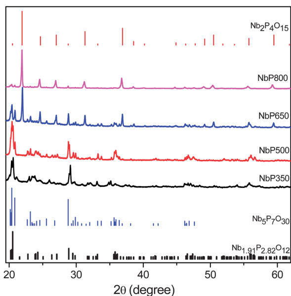
Fig. 1 XRD patterns of niobium phosphates sintered at different temperatures as indicated in the figure.
