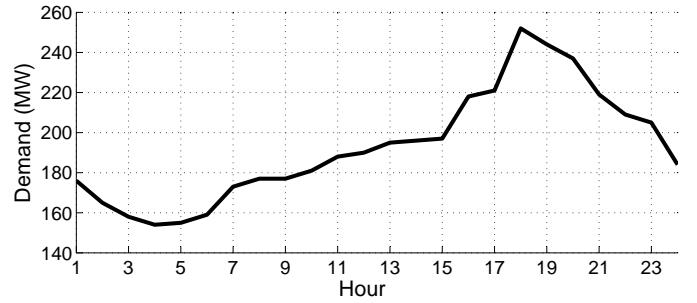
Figure 1. Demand over 24 hours, (\sum_d P_{d,t}^{max}, \forall t)
