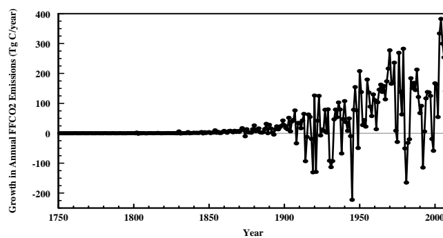
Fig. 3b. Growth of FFCO 2 emissions from the year 1752 to 2007. Positive values indicate an increase in year-to-year emissions and negative values indicate a decrease in year-to-year emissions. A gray zero line has been added for reference. Data from Boden et al. (2010).
