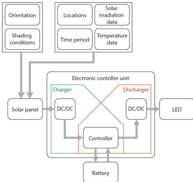
Fig. 4. Block diagram of L2L modelling tool.
