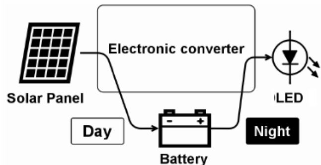
Fig. 2. Working principle of the converter
