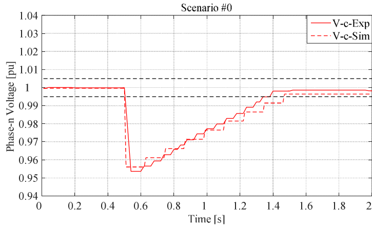
Fig. 6. Tap actions for phase c for Scenario #0
