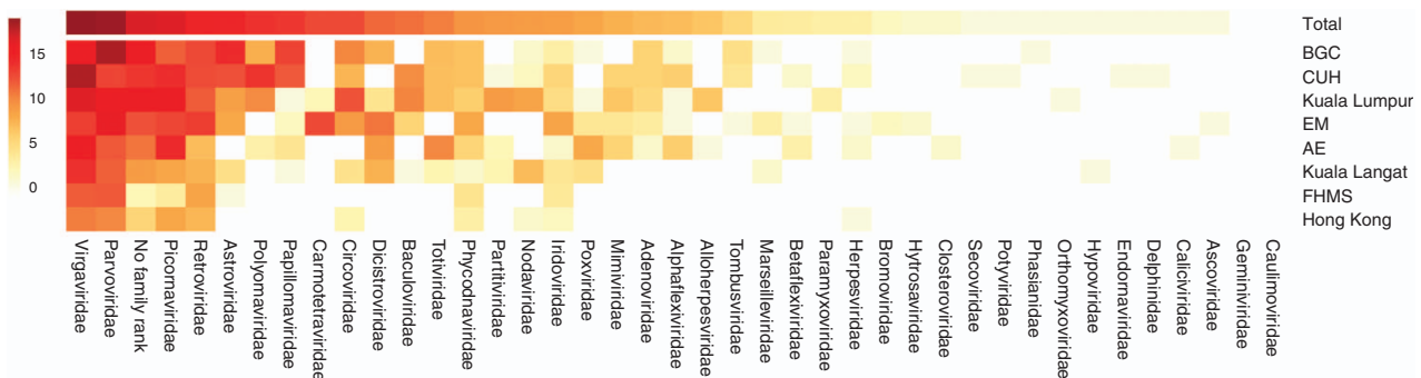
Figure 3 Abundance and diversity of virus families. Distribution and taxonomic classification (family) of reads mapping to assembled viral contigs. Colour intensity represents \log_2 -transformed counts of reads mapped to the contigs resembling a viral family for each sampling location shown on the y-axis. Sample locations in Denmark are abbreviated as indicated: Amager East (AE), Egedal (EM), Botanical Garden of Copenhagen (BGC), Faculty of Health and Medical Sciences (FHMS) and Copenhagen University Hospital (CUH).
