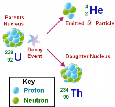
Figure 1.2. Decay of a uranium-238 nucleus through emission of an alpha particle (helium nucleus).
