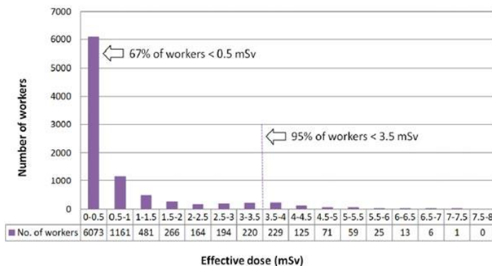
Figure 1.10. Annual dose effective distribution for all Australian uranium mine workers in 2013.
