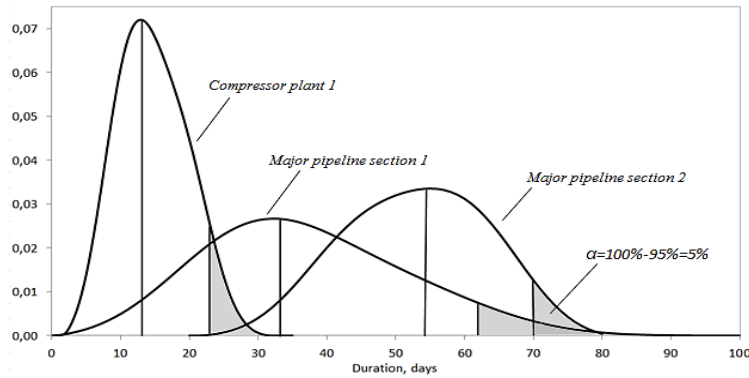
Figure 2. Pdfs of Repair Projects' Durations
