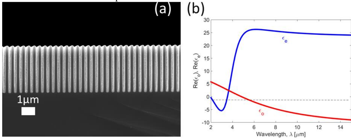
Fig. 1: (a) Electron micrograph image of fabricated Al-doped ZnO (AZO) structures between Si trenches with high aspect ratio. (b) Effective ordinary and extraordinary permittivities, \epsilon_o and \epsilon_e of the AZO trench structure based on effective media approximation, showing the hyperbolic properties of the structure for wide range of mid-infrared wavelength region.
