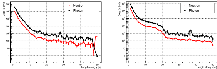
Figure 8: Histograms showing the dose rate along the straight (left) and curved (right) example guides described in section 4. Only neutrons in the wavelength range: 0.5 \text{ \AA} - 1.0 \text{ \AA} are accounted for. Energy- and particle dependent conversion factors have been applied when converting from fluence to effective dose in accordance with Swedish radiation protection authorities[17, 18].
